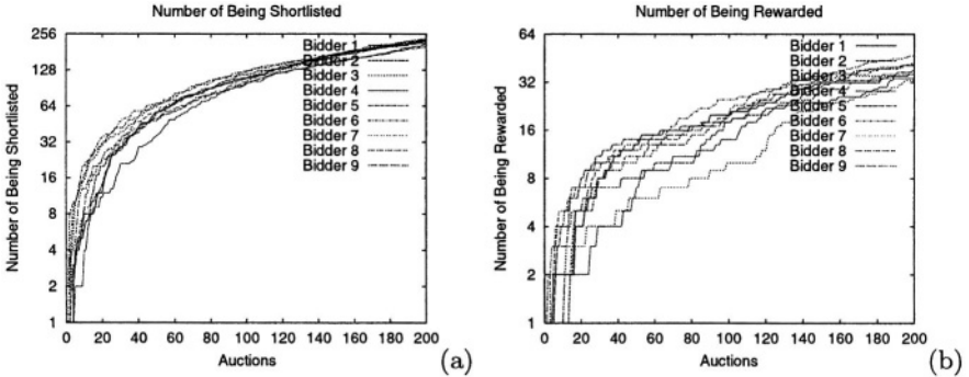
Fig. 9. Opportunity of Being Shortlisted and Rewarded.
