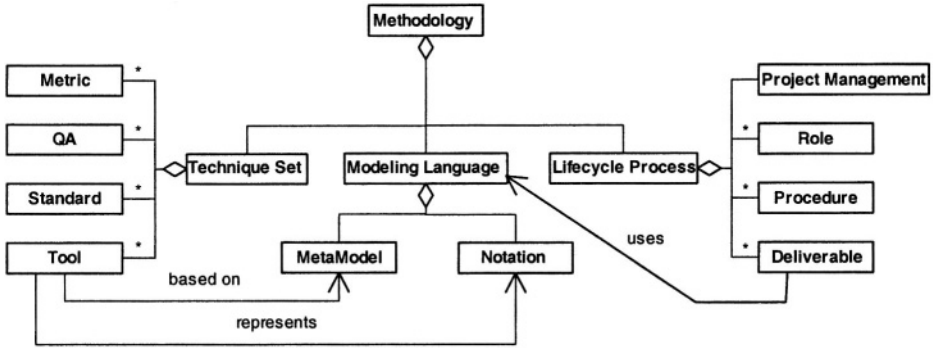
Fig. 1. The components of a methodology and the relationships among them.
