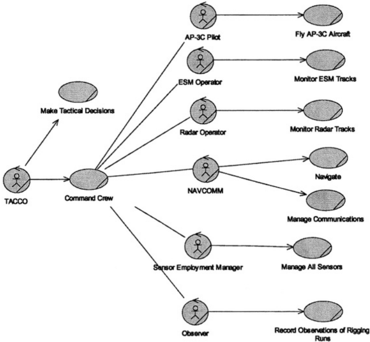
Fig. 2. Representation of a partial domain model in UML. This diagram shows the roles and relationships between the members of the crew on-board an AP-3C aircraft. This domain model is a store of knowledge that can be referenced to construct the agent models.
