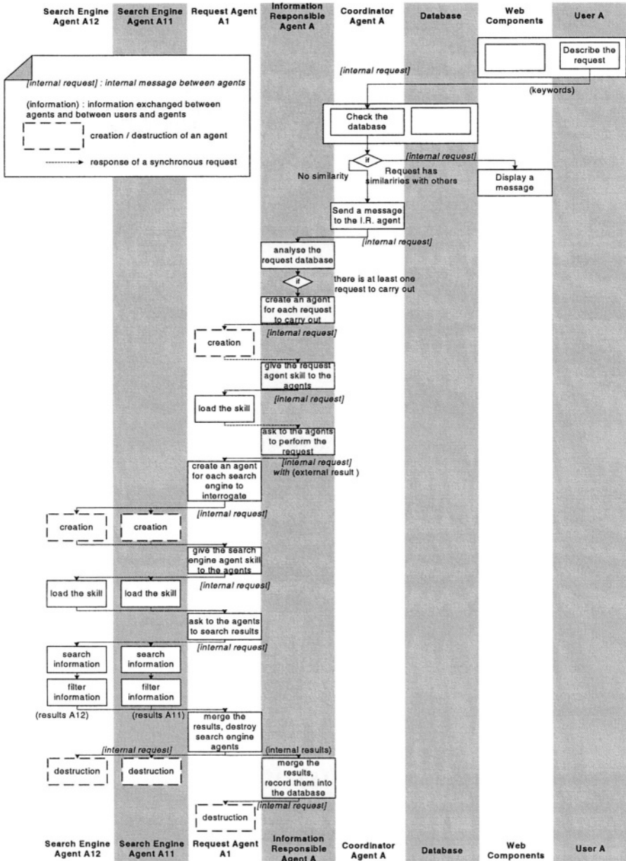
Fig. 4. Processing model of the request recording process in a CIASTWA.
