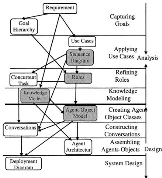
Fig. 2. E i - MaSE Steps and Models.
