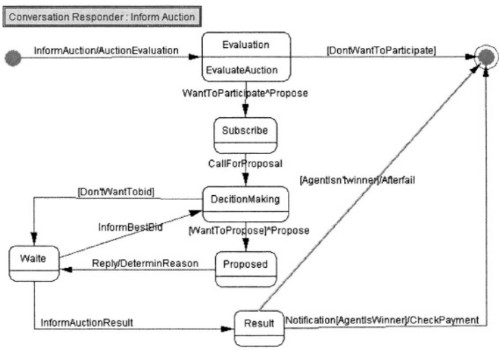
Fig. 9. Inform Auction Task Diagram of the CASBA System.
