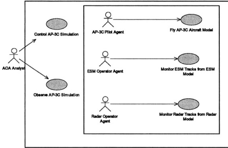
Fig. 4. A use case diagram for the representing behaviours in an AP-3C simulator, for both an analyst and agents in the virtual environment. The outer box represents the simulation software system. The inner box represents the virtual environment. This diagram extends the normal UML representation of actors to represent agents within the simulation system.
