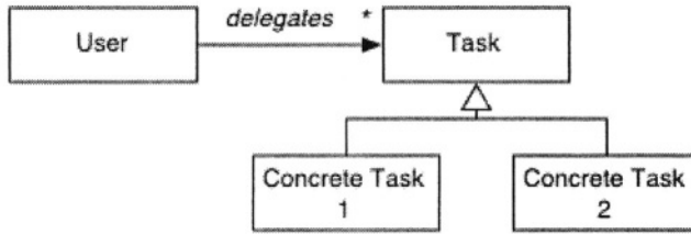
Fig. 3. Role diagram for AGENT AS DELEGATE.
