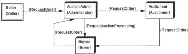
Fig. 12. Deployment Diagram of the CASBA System.
