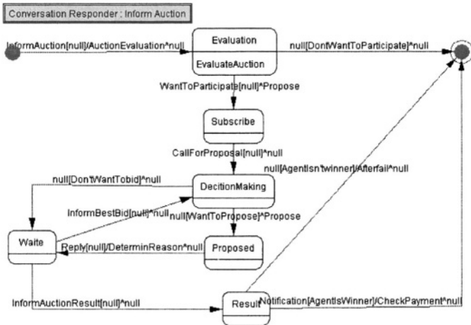
Fig. 11. Inform Auction Conversation (Responder).
