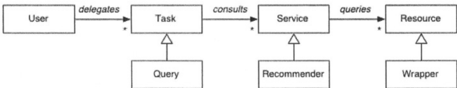
Fig. 7. Architecture after applying AGENT AS MEDIATOR.
