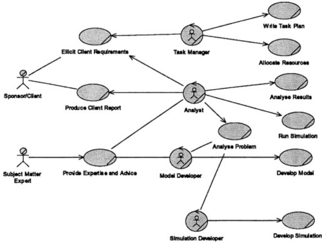
Fig. 1. A diagrammatic representation of part of a business model for Air Operations Analysis branch using UML. The sponsor/client are air force officers that will make use of the advice provided from by the branch. The subject matter experts (SME) are typically the operational crews of the aircraft and the engineers experienced in the technical aspects of the on-board systems.
