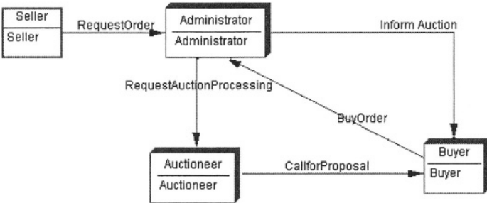
Fig. 10. Agent-object Class Diagram of the CASBA System.
