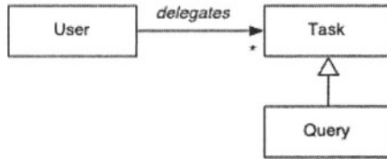
Fig. 6. Initial architecture after applying AGENT AS DELEGATE.
