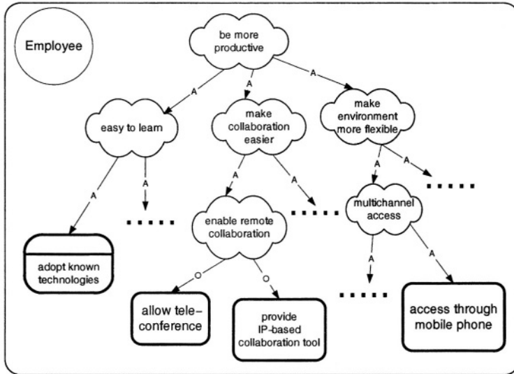
Fig. 7. The “be more productive” Soft-Goal Model.
