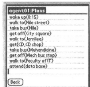
Fig. 6. Plan incorporating both user goals.
