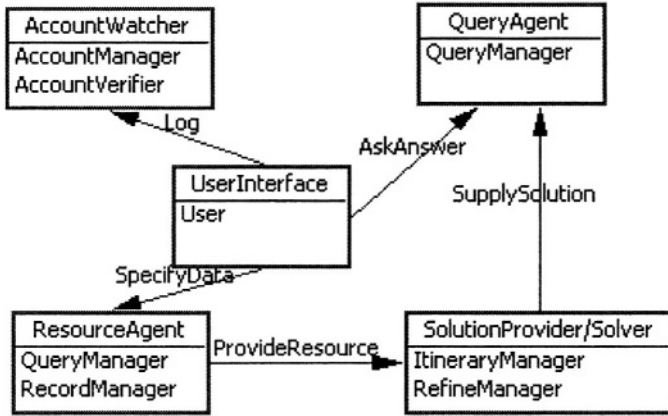
Fig. 1. PIPS agent class diagram (extracted from the PIPS design documentation produced by Yenty Frily using agentTool).
