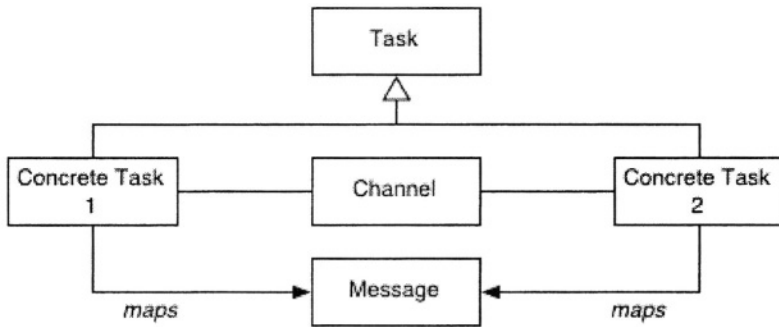
Fig. 5. Role diagram for COMMON VOCABULARY.
