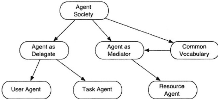
Fig. 1. Roadmap for the pattern language.
